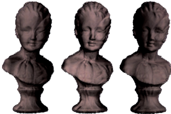
Figure 10: 42 \times 42 PTM light field with fixed view direction and light position moving from left to right.
