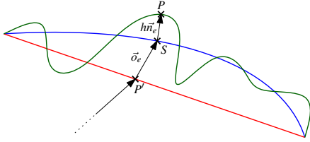
Figure 5: Computation of camera-centric coordinates. P' is interpolated from the quad corners along the red line. The displacement vector \vec{o}_e is the offset between P' and the corresponding position S on the ellipsoid surface (blue). The final position P on the true surface geometry (green) is computed by applying the elevation h along the normal \vec{n}_e .
