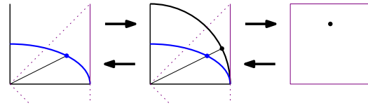
Figure 2: Forward and inverse map projection. For forward projection, a point on the reference ellipsoid (left) is first shifted to the sphere (middle), and then projected onto the cube side (right).
