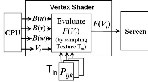
Fig. 3. The Single-Phase (SP) HFFD algorithm that is executed solely on the vertex processor.
