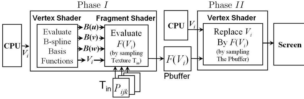
Fig. 4. The double phase (DP) algorithm for HFFD. The algorithm employs both the vertex processor and the pixel processor to compute F .
