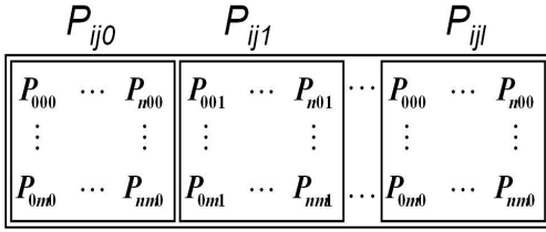
Fig. 2. A three-dimensional lattice of control points of F , laid out in a two-dimensional floating point texture map, T_{in} .
